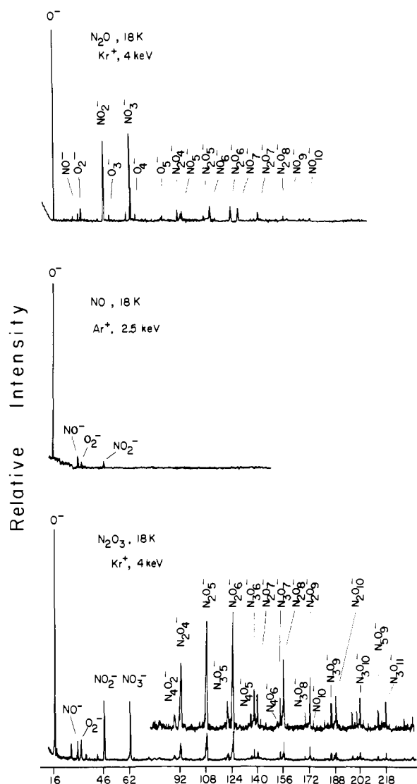
Figure 13. The negative SIMS of solid N_2O and N_2O_3 , using Kr^+ at 4 keV as the projectile ion, and of solid NO , using Ar^+ at 2.5 keV as the projectile ion.
