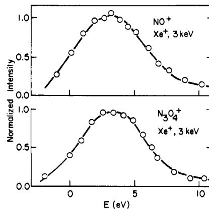
Figure 4. The energy distribution of positive secondary ions of solid NO with Xe^+ at 3 keV as the primary ion. The horizontal scale contains an unknown additive constant.
