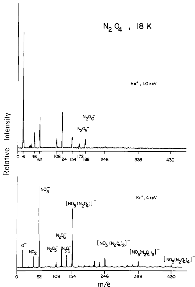
Figure 2. The negative secondary ion mass spectra of solid N_2O_4 with He^+ as the primary ion at 1 keV and Kr^+ as the primary ion at 4 keV.
