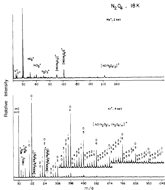
Figure 9. Positive SIMS of solid N_2O_4 with He^+ at 2 keV and Kr^+ at 4 keV as the projectile ion.
