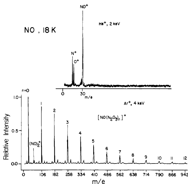
Figure 7. Positive SIMS of NO with He^+ at 2 keV and Ar^+ at 4 keV as the projectile ion.
