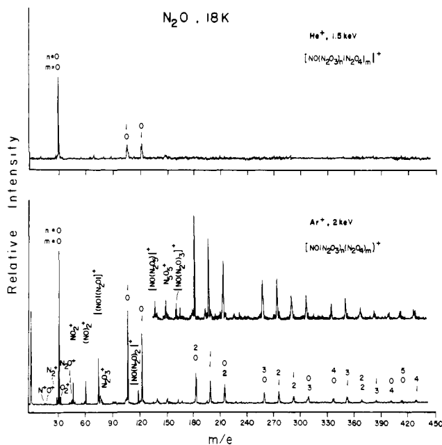
Figure 6. Positive SIMS of N_2O with He^+ at 1.5 keV and with Ar^+ at 2 keV as the impacting ion.
