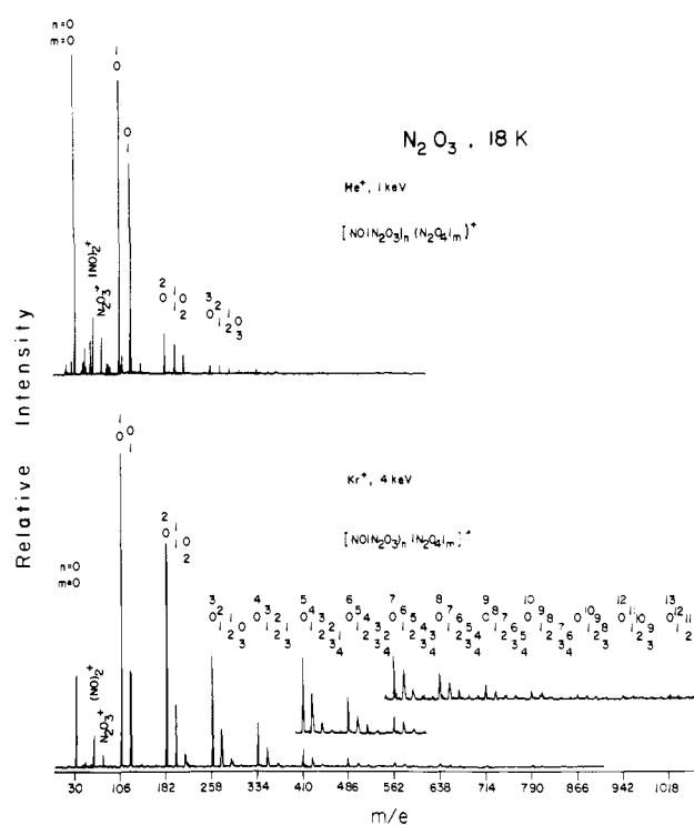
Figure 8. Positive SIMS of N_2O_3 with He^+ at 1 keV and Kr^+ at 4 keV as the impacting ion.
