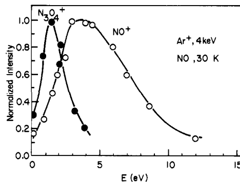
Figure 3. The energy distribution of positive secondary ions of solid NO with Ar^+ at 4 keV as the primary ion. The horizontal scale contains an unknown additive constant.
