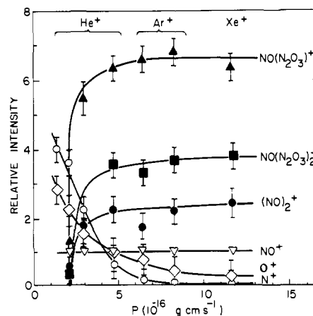
Figure 1. Relative intensity of positive secondary ions from solid NO as a function of the momentum of the primary projectile.
