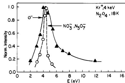
Figure 5. The energy distribution of negative secondary ions of solid N_2O_4 with Kr^+ at 4 keV as the projectile ion. The horizontal scale contains an unknown additive constant.
